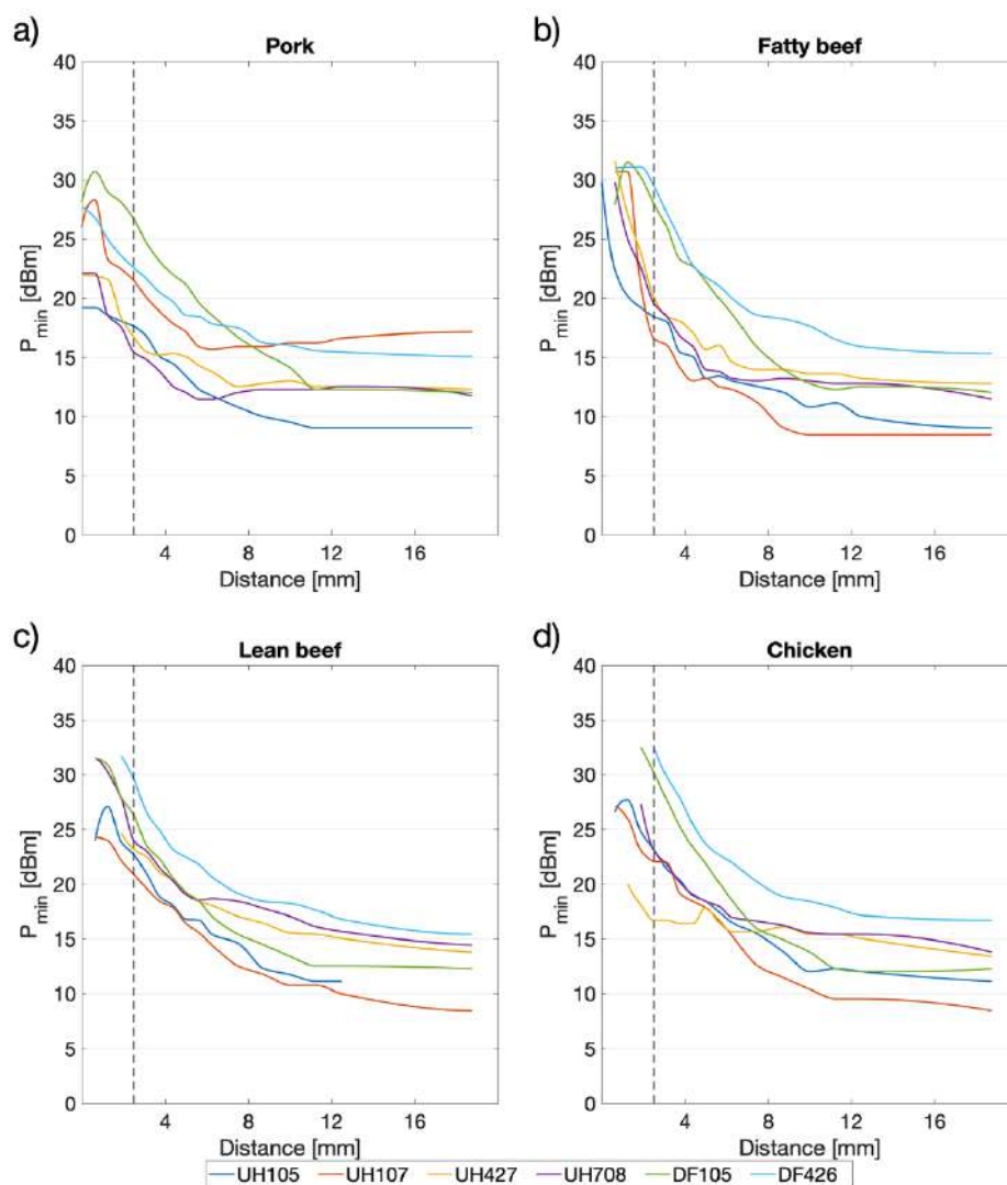
Figure 4. Mean values of the minimum power required to activate the UHF and DF tags ( P_{\min} (dBm)) at increasing tag-to-meat distances (mm) when tested on different types of minced meat patties. The dashed lines highlight the minimum distance at which all the six tags were detected. Subfigure (a) regards pork, Subfigure (b) regards fatty beef, Subfigure (c) regards lean beef, while Subfigure (d) regards chicken.
