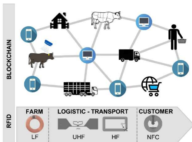
Figure 1. Example of meat supply-chain digitalisation. The Low Frequency (LF) ear-tag contains the animal code which is registered in private and public repositories. High Frequency (HF) and Ultra-High Frequency (UHF) tags identify meat cuts, and Near Field Communication (NFC) tags are used on packed meat in retail. The distributed and decentralised data infrastructure using blockchain enhances the level of trust in the traceability system.
