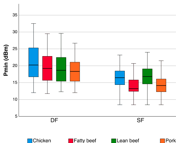
Figure 5. Comparison of the Single Frequency (SF) and Dual Frequency (DF) tag types on four meat types when detection is performed in the UHF band. The data are expressed as the minimum power required to activate the tags ( P_{\min} (dBm)) on a box-plot graph. The tag types are compared in the 2.5–18.75 mm range of distances.
