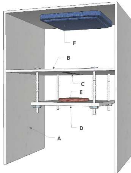
Figure 2. UHF test bench: (A) low-density polystyrene box, (B) central fixed shelf, (C) UHF tag, (D) adjustable platform, (E) meat sample and (F) UHF panel antenna.
