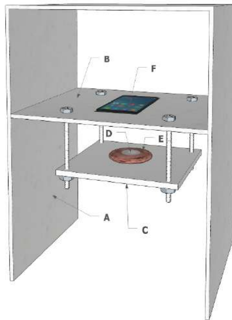
Figure 3. HF test bench: (A) low-density polystyrene structure, (B) central fixed shelf, (C) adjustable platform, (D) NFC tag, (E) meat sample and (F) Android smartphone embedding the NFC reader.
